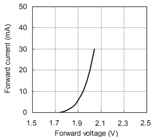
伏安特性曲线 Forward Current vs. Forward Voltage
