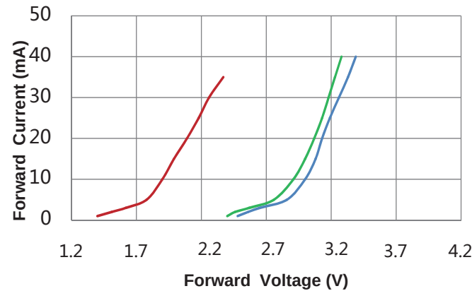
伊守滴怱早筌 Forward Current VS. Forward Voltage (Ta=25°C)
