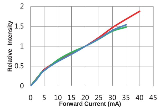
瓶寸先弹不特沃滴怱早筌 Relative Intensity VS. Forward Current (Ta=25°C)
