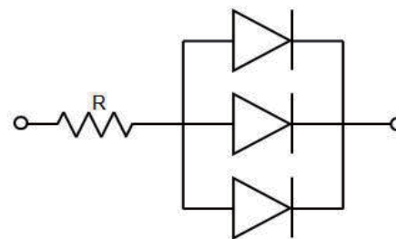
特瑶桑弄/ Circuit model B
