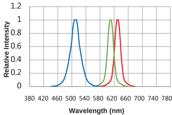
先谱刀市滴怱早筌 Spectrum Distribution (Ta=25°C)
