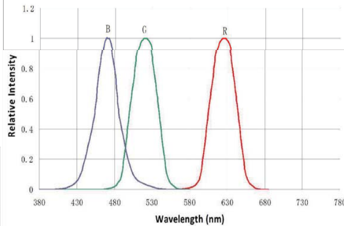
Spectrum Distribution ( T_a=25^\circ\text{C} )
