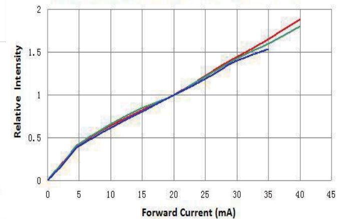
Relative Intensity VS. Forward Current ( T_a=25^\circ\text{C} )
