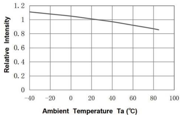
Relative Intensity VS. Ambient Temperature ( T_a=25^\circ\text{C} )
