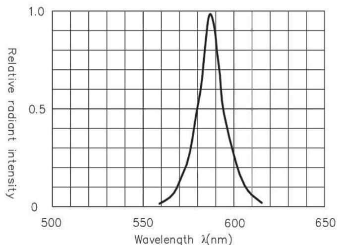
光谱分布曲线 Relative Intensity Vs. Wavelength
