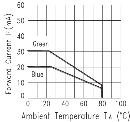
Derating Curve
