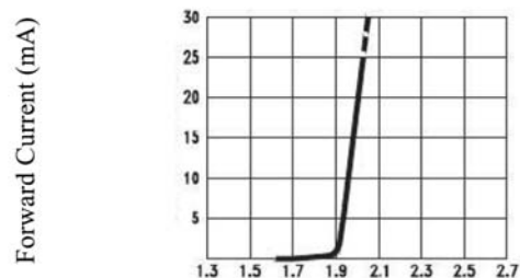
伏安特性曲线 Forward Current VS. Forward Voltag (Ta=25°C)
