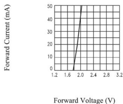
伏安特性曲线 Forward Current VS. Forward Voltage (Ta=25°C)
