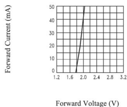
伏安特性曲线 Forward Current VS. Forward Voltag (Ta=25°C)
