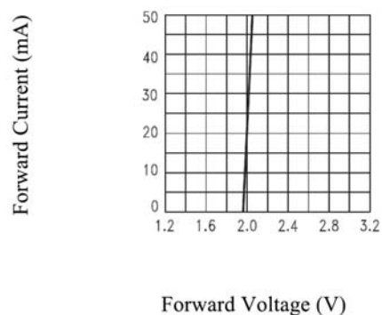
伏安特性曲线 Forward Current VS. Forward Voltag (Ta=25°C)
