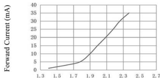
伏安特性曲线 Forward Current VS. Forward Voltag (Ta=25°C)
