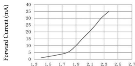
伏安特性曲线 Forward Current VS. Forward Voltage (Ta=25°C)
