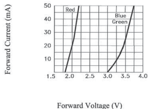
伏安特性曲线 Forward Current VS. Forward Voltage (Ta=25°C)
