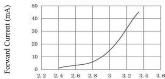
伏安特性曲线 Forward Current VS. Forward Voltag (Ta=25°C)
