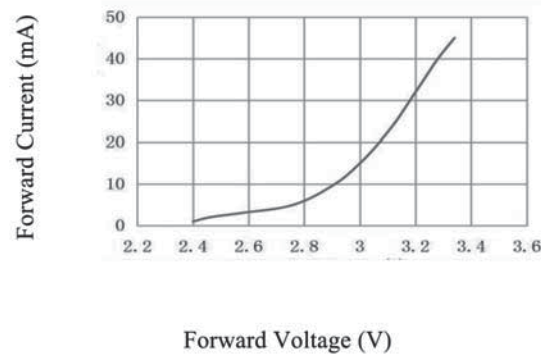
伏安特性曲线 Forward Current VS. Forward Voltag (Ta=25°C)
