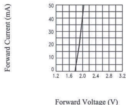
伏安特性曲线 Forward Current VS. Forward Voltage (Ta=25°C)
