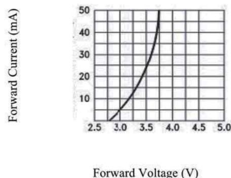
伏安特性曲线 Forward Current VS. Forward Voltage (Ta=25°C)
