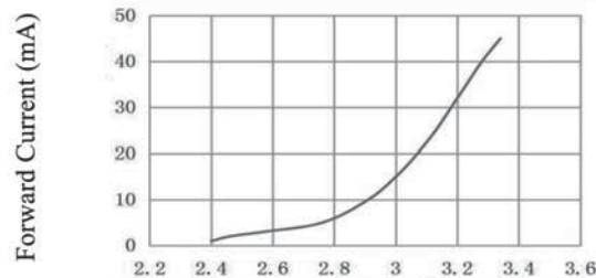
伏安特性曲线 Forward Current VS. Forward Voltage (Ta=25°C)
