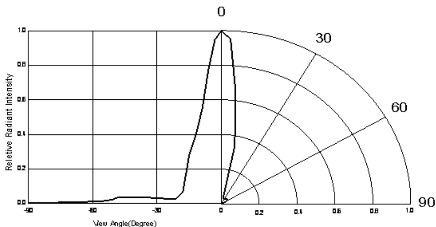
Relative Radiant Intensity vs. Angular Displacement
