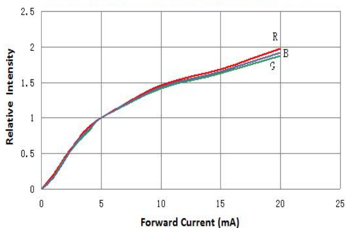
Relative Intensity VS. Forward Current (Ta=25°C)
