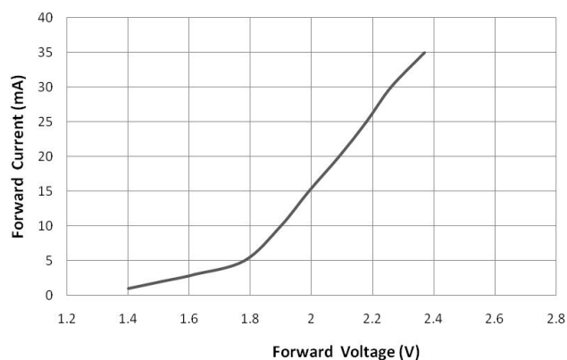
Forward Current VS. Forward Voltage (Ta=25℃)
