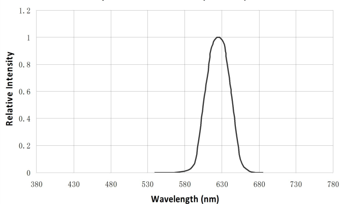
Spectrum Distribution (Ta=25℃)
