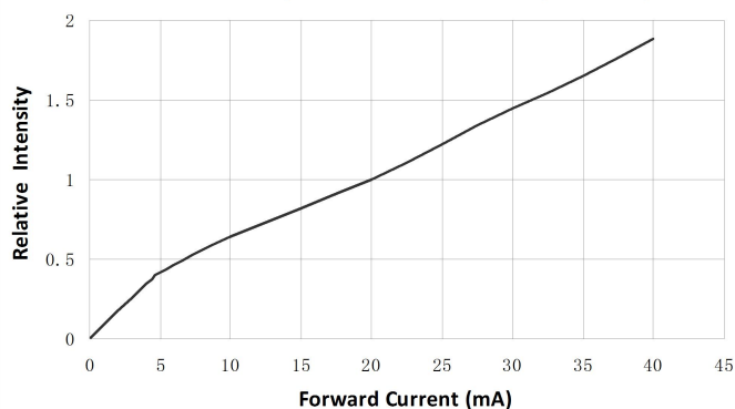
Relative Intensity VS. Forward Current (Ta=25℃)
