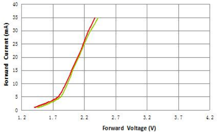
Forward Current VS. Forward Voltage ( T_a=25^{\circ}\text{C} )
